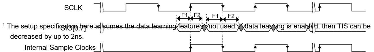
Figure 38. FlexSPI input timing in DDR mode where FlexSPIn_MCR0[RXCLKSRC] = 0x0, 0x1
