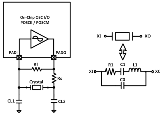
Figure 5. Crystal model and external components
