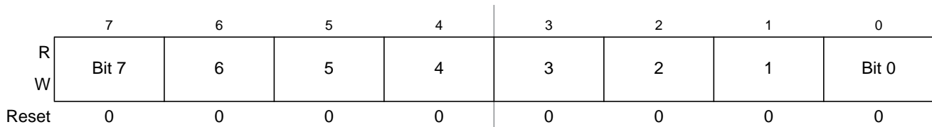
Figure 10-14. TPM Channel Value Register Low (TPMxCnVL)
